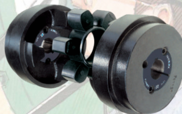
HRC Couplings
